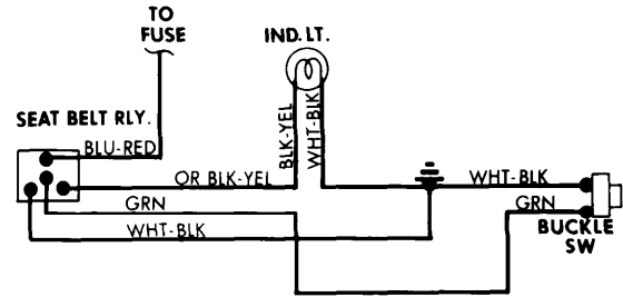
Seat Belt Warning System Wiring Diagram (Toyota Land Cruiser)
