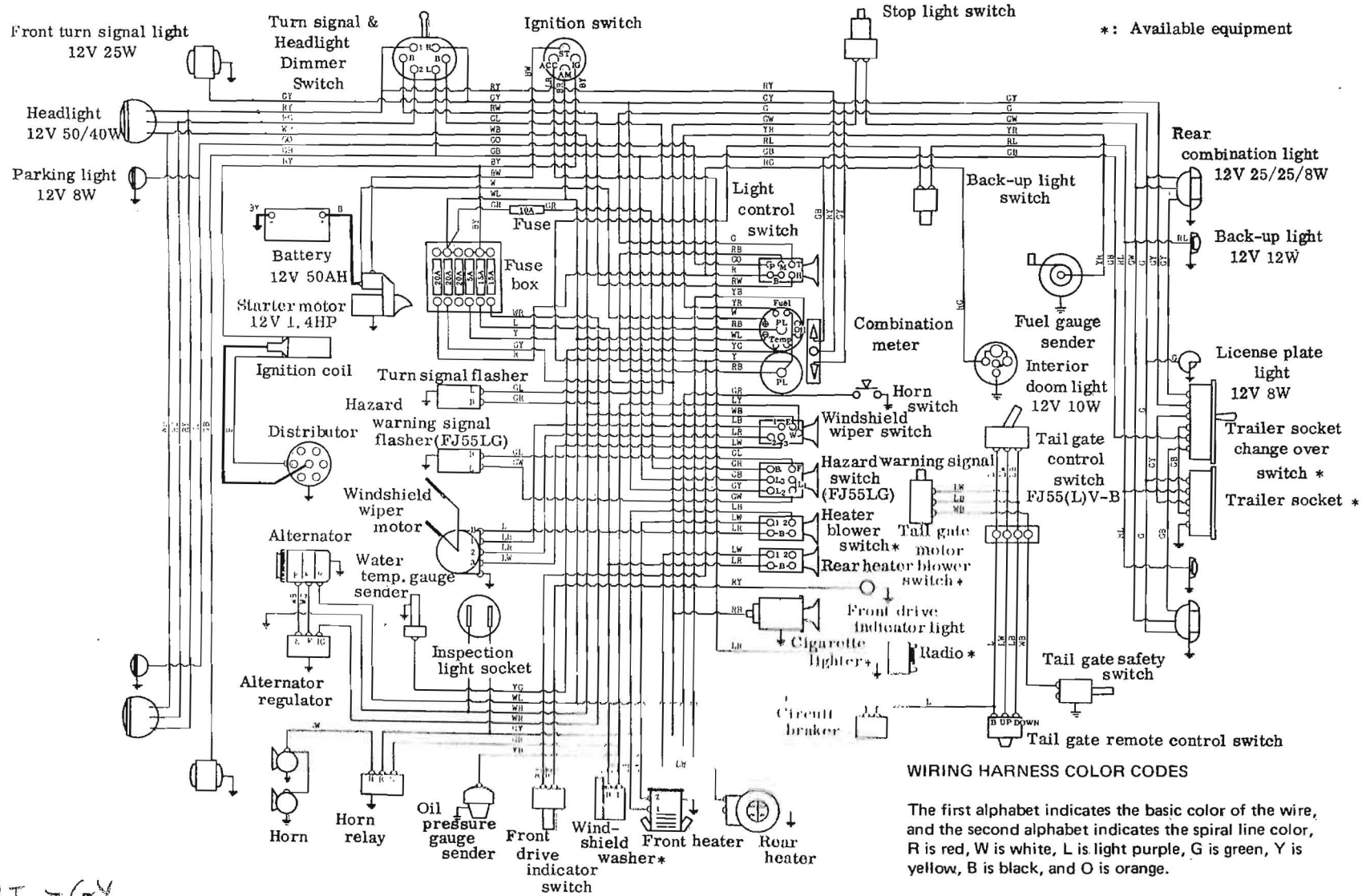
Fig. 11.68. Wiring diagram - FJ55 series, pre-1972 (early)
